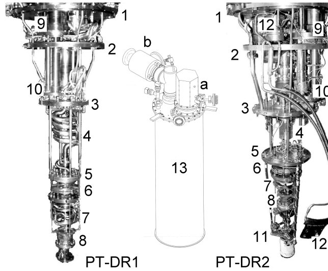
Fig. 1. 1: 300 K flange, 2: 60 K flange, 3: 4 K flange, 4: vapor (700 mK/4 K) exchanger, 5: still, 6: continuous exchanger, 7: step exchangers, 8: mixing chamber, 9: PT1, 10: PT2, 11: nuclear demagnetization, 12: N 2 thermal pipe, 13: global view of PT(a) and pumping line(b).
