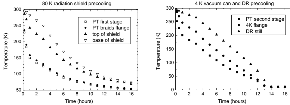
Fig. 2. Typical PT-DR2 pre-cooling curves.
