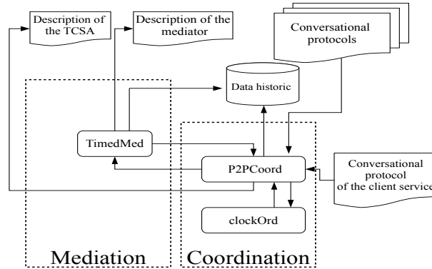
Fig. 7 Underlying architecture of the prototype.
