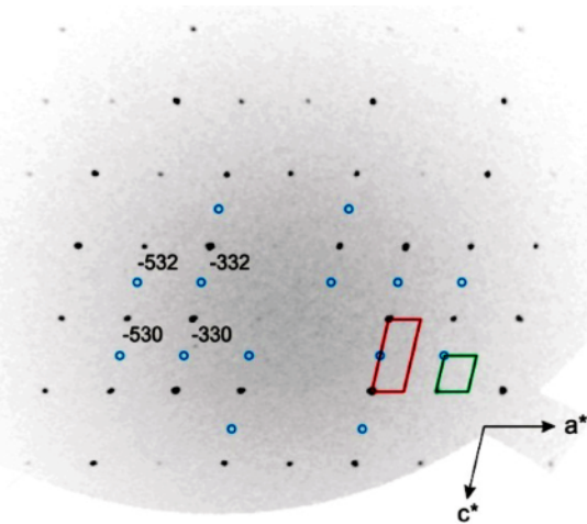
Fig. 1 (color online). The reciprocal layer h3l calculated from the diffractometer data set (integrated for the 2c superstructure cell). The unit cells of the subcell (red) and the superstructure (green) are given. Blue circles denote positions of (not detected) superstructure reflections.
