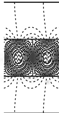
Fig. 3. Streamlines (continuous lines) and isotherms (dashed lines) for d = \delta = \alpha = Pe = 1 . Showing the effect of having different wavenumbers.
