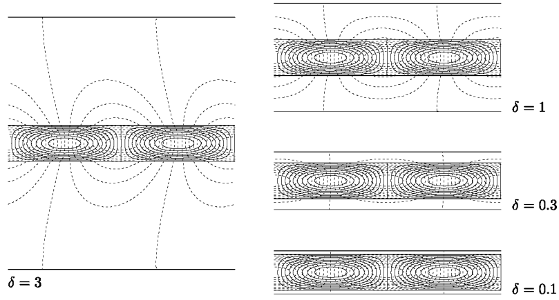
Fig. 5. Streamlines (continuous lines) and isotherms (dashed lines) for \alpha = \text{Pe} = 1 and d = 5 . The wavenumber is k = 1 . Showing the effect of having different values of \delta .
