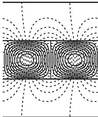
Fig. 3. Streamlines (continuous lines) and isotherms (dashed lines) for d = \delta = \alpha = Pe = 1 . Showing the effect of having different wavenumbers.
