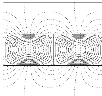
Fig. 3. Streamlines (continuous lines) and isotherms (dashed lines) for d = \delta = \alpha = Pe = 1 . Showing the effect of having different wavenumbers.
