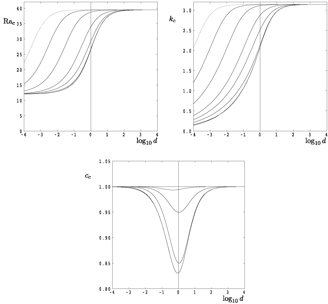
Fig. 11. Critical values for Ra_c , k_c and c_c as a function of d for \alpha = Pe = 1 and for \delta = 10^{-4}, 10^{-3}, 10^{-2}, 10^{-1}, 10^{-0.5}, 10^0, 10^{0.5}, 10^1 and 10^2 . The dotted line corresponds to \delta = 10^{-4} .
