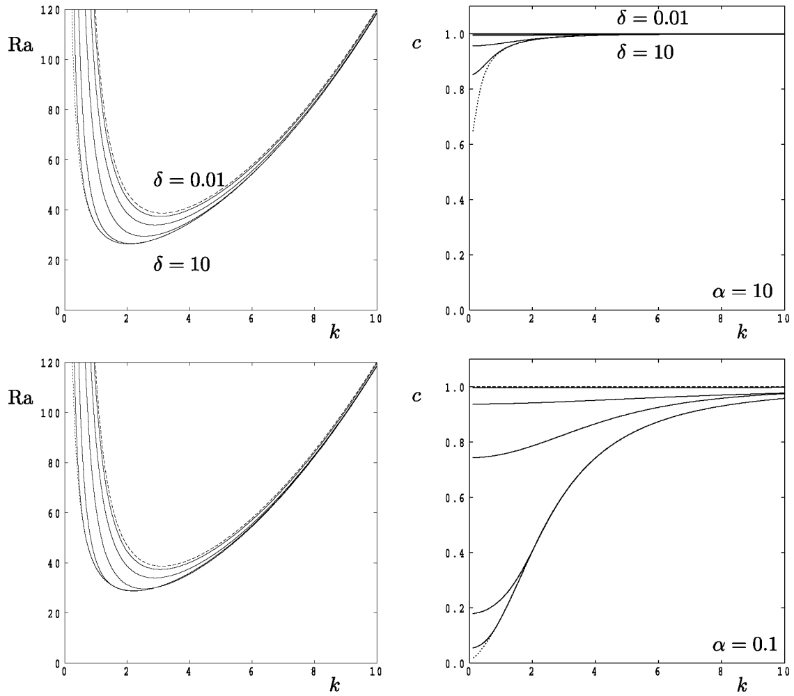
Fig. 6. Neutral curves (left) and the corresponding values of the wavespeed, c , (right) for d = 1 and \text{Pe} = 1 for the stated values of \alpha . The following values of \delta were used: \delta = 10, 3, 1, 0.3, 0.1, 0.03 and 0.01 . The dotted line corresponds to \delta = 10 and the dashed line to \delta = 0.01 .
