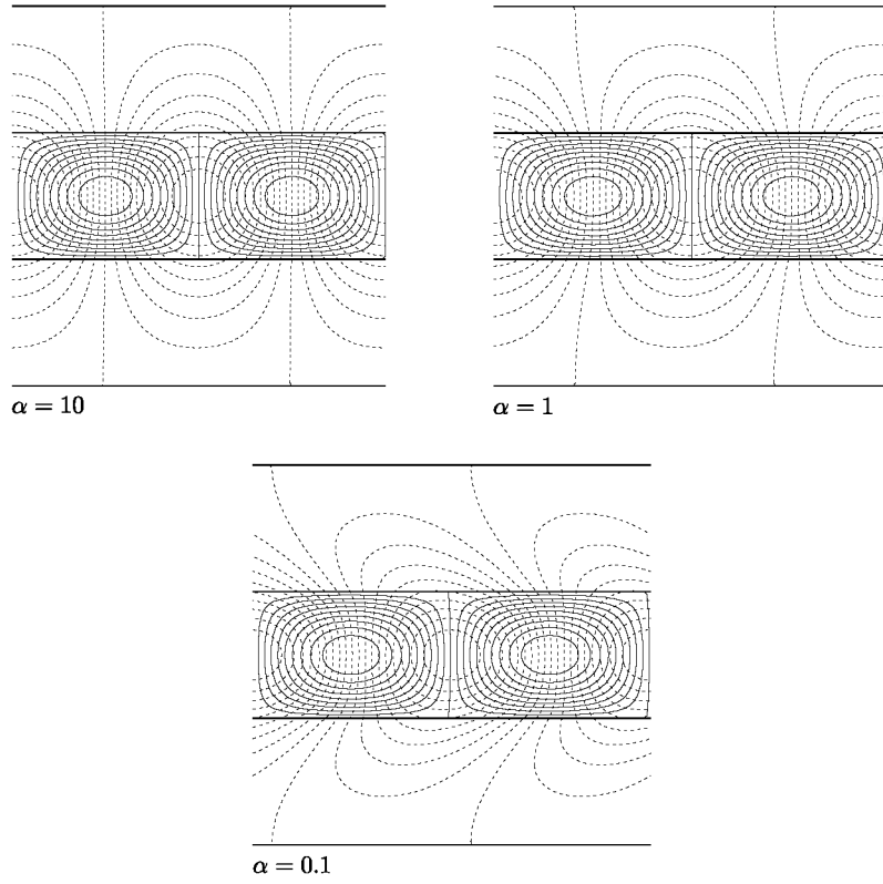
Fig. 7. Streamlines (continuous lines) and isotherms (dashed lines) for \delta = d = \text{Pe} = 1 . The wavenumber is k = 2 . Showing the effect of having different diffusivity ratios, \alpha .
