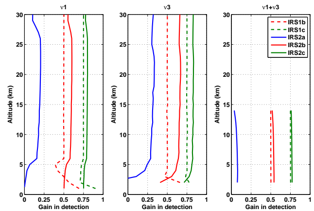
Figure 15. Impact study on the detection limit for SO 2 . The plot represents the relative difference ratio between the detection limit of each scenario and the IRS1a-IASI scenario, as a function of altitude, for a case representative of a tropical atmospheric situation, when using the \nu_1 band (left), \nu_3 band (middle) and the \nu_1 + \nu_3 band (right). Note that the sensitivity of the latter band is limited to under 15 km.
