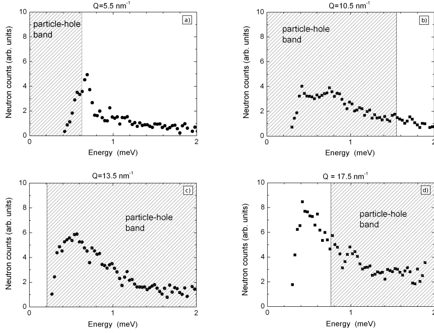
Fig. 1. Dynamic structure factor of two-dimensional {}^3\text{He} , obtained from inelastic neutron scattering at 4 different wave vectors Q and an areal density of 4.9\text{ nm}^{-2} . The shaded area is the particle-hole continuum. Note the strong peak below it in the lower right figure.
