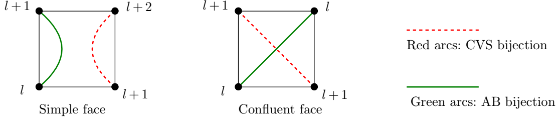
Figure 1: Convention for adding arcs in the bijections.
