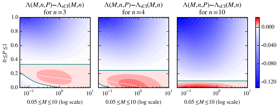
Fig. 9 (M, P) \mapsto \Delta(M, n, P) - \Lambda_{sCI}(M, n) for n = 3 (left), n = 4 (center) and n = 10 (right). The red zones correspond to \mathcal{P}_{M,n} . The upper and lower green curves correspond to the roots P' = P'(M, n) (lower curve) and P'' = 1/n (upper curve) of \Delta(M, n, P) - \Lambda_{sCI}(M, n) = 0 . The central white curve shows M \rightarrow P^*(M, n) (Color figure online)
