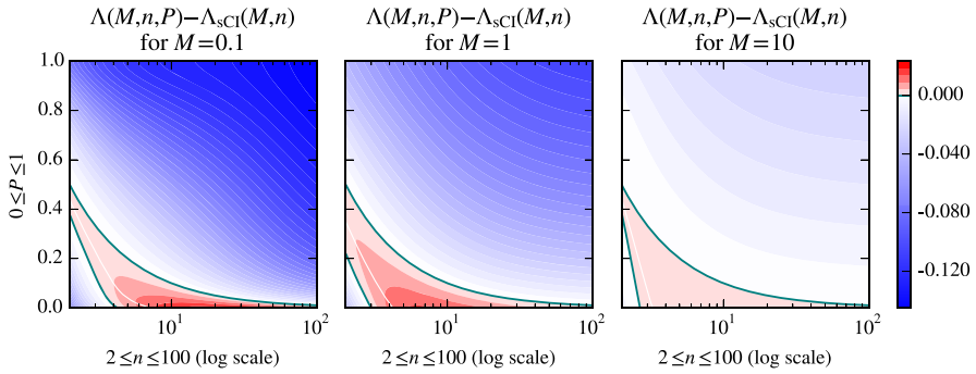
Fig. 8 (n, P) \mapsto \Delta(M, n, P) - \Lambda_{sCI}(M, n) for M = 0.1 (left), M = 1 (center) and M = 10 (right). The red zones correspond to \mathcal{P}_{M,n} . The upper and lower green curves correspond to the roots P' = P'(M, n) (lower curve) and P'' = 1/n (upper curve) of \Delta(M, n, P) - \Lambda_{sCI}(M, n) = 0 . The central white curve shows n \rightarrow P^*(M, n) (Color figure online)
