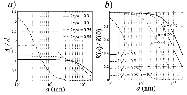
Fig. 9 (a) Ratio of Washburn prefactor corrected for the presence of bubbles to the classical Washburn prefactor as a function of the slit aperture for several bubble sizes and a slit width of 3 \mu\text{m} . (b) Ratio between K(\varepsilon) and the permeability of a Hele-Shaw slit K(0) for the same set of parameters as for (a).
