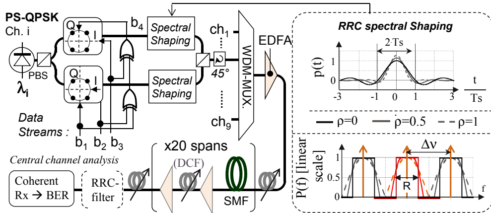
Fig. 1. Simulation setup for our transmission system including RRC spectral shaping description. p(t) is the fundamental pulse in the case of RRC spectral shaping.
