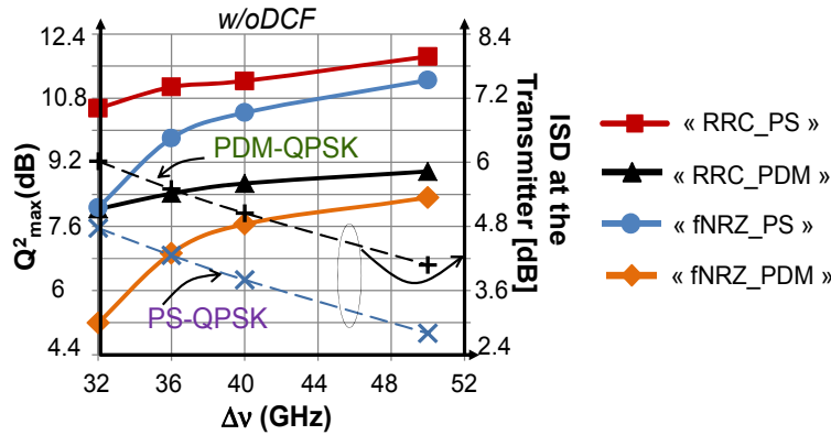
Fig. 3. Q^2_{\max} as a function of the channel spacing \Delta\nu in the “w/oDCF” case for all the considered modulation format solutions.
