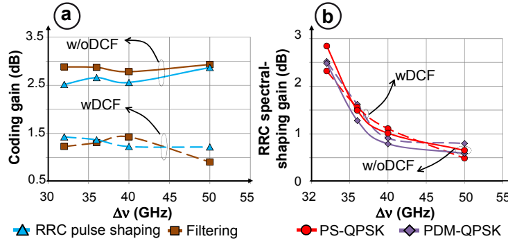
Fig. 4. “Coding gain” (a) and “RRC spectral shaping gain” (b) as a function of the channel spacing \Delta v in the “w/oDCF” (solid lines) and in the “wDCF” DC scheme (dashed lines).
