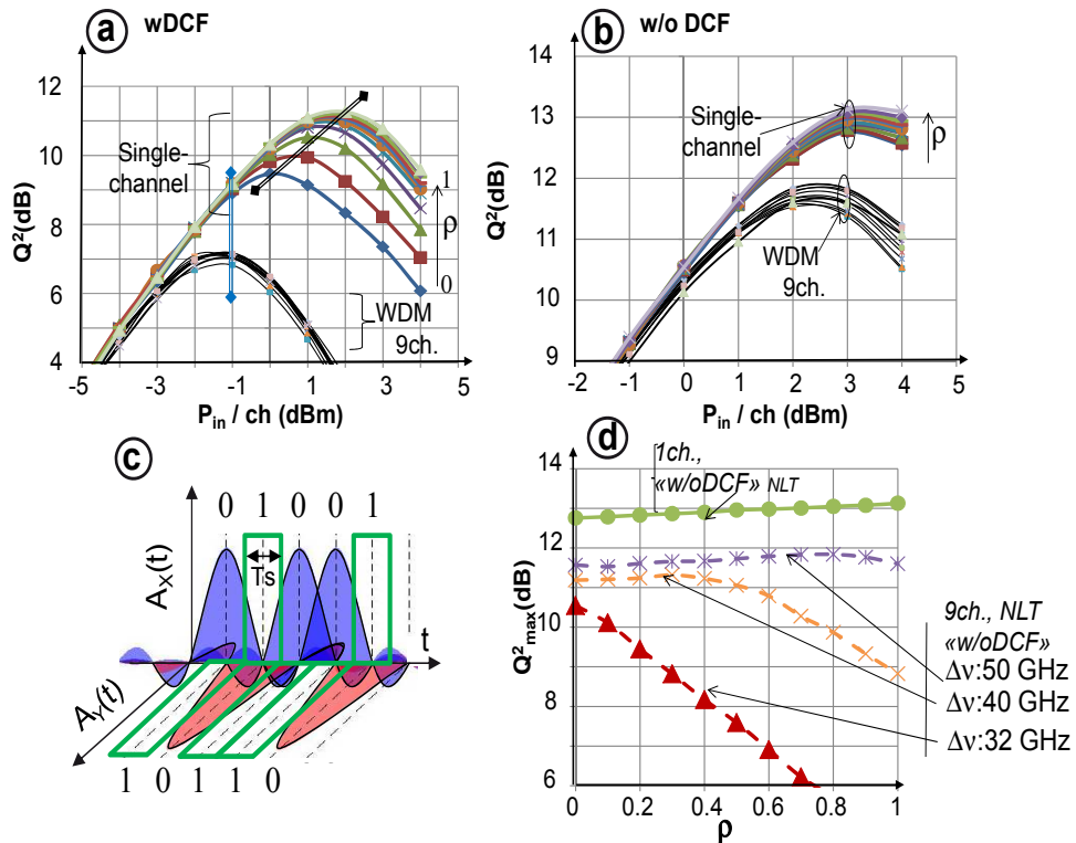
Fig. 2. Q^2 versus P_{in,avg} for “RRC_PS” with different roll-off factors for either 1 or 9 channels ( \Delta\nu = 50 GHz) in the scenarios “w/DCF” (a) and “w/oDCF” (b). Illustration of adjacent, spectrally-shaped RRC pulses, in the context of polarization switching (c). Q^2_{\max} as a function of \rho (d) for 1 (solid line) or 9 channels (dashed line) in the case “w/oDCF”.
