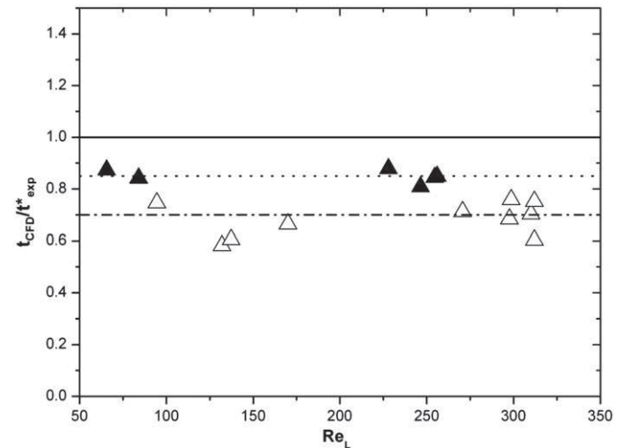
Fig. 8. Exposure time versus the liquid Reynolds number. Comparison between present work and (—) Raynal et al. (2008); (- -) present work: Eq. (18) for K=0.85 ; (- ● -) present work: Eq. (18) for K=0.7 .
