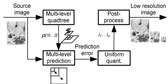
Fig. 1. Flat coder schemes
