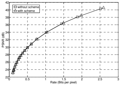
Fig. 12. LAR PSNR performance on p06
