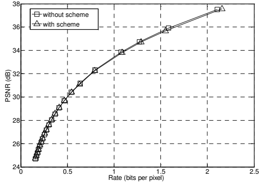
Fig. 11. LAR PSNR performance on bike
