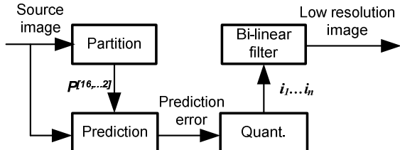
Fig. 2. Flat coder schemes
