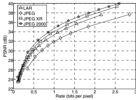
(a) PSNR performances on bike
