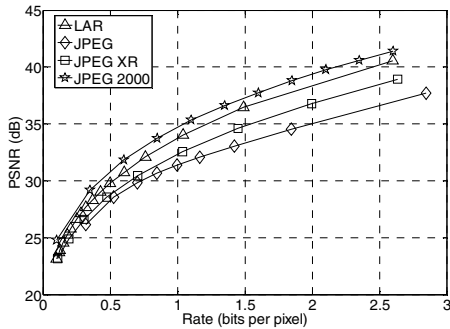
(b) PSNR performances on p06
