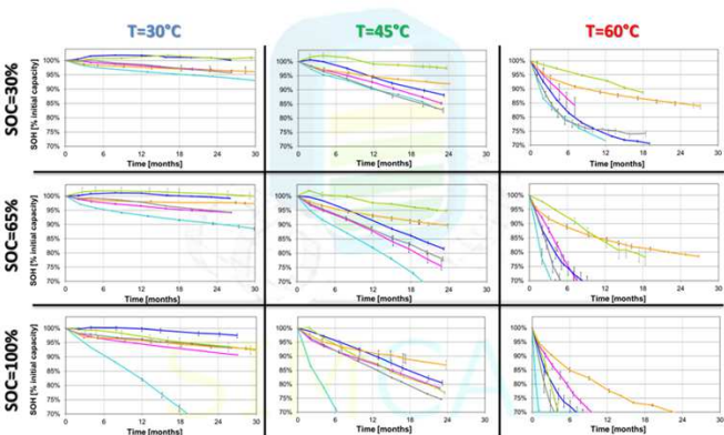
Fig. 1: Calendar aging measured on 6 Li-ion commercial cells according to 9 aging conditions (measured data)
