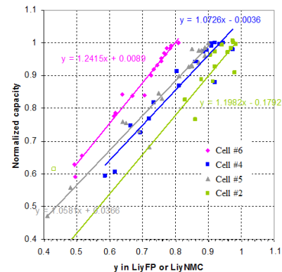
Fig. 2: Cells capacity fade vs. cathodes maximum Li stoichiometry
