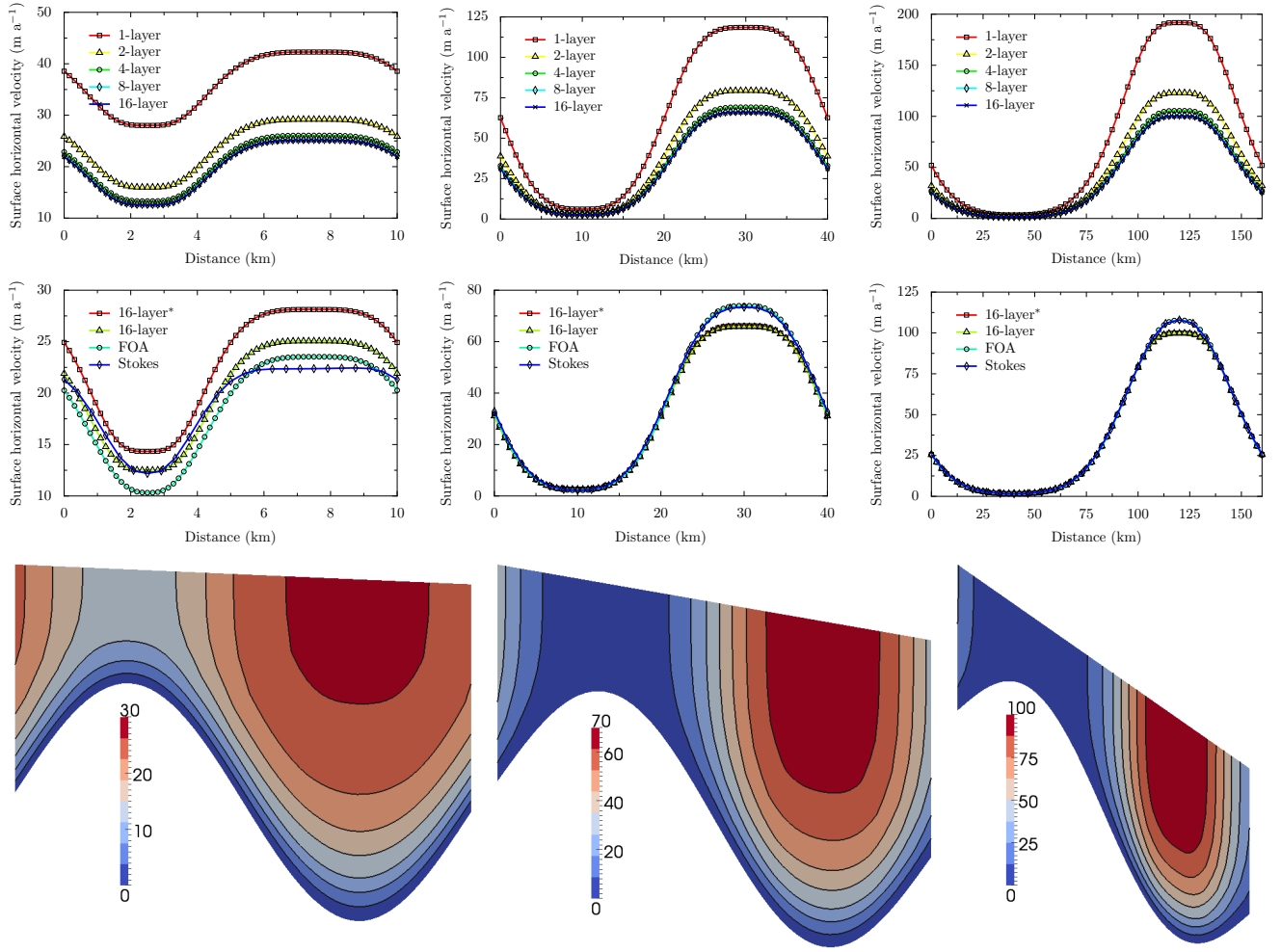
Figure 5: ISMIP-HOM Experiment B results for L_x = 10, 40 and 160 km, from left to right, respectively. Top: surface horizontal velocities of the 1-layer, 2-layer, 4-layer, 8-layer, and the 16-layer models. Middle: surface horizontal velocities of the 16-layer*, the 16-layer, the FOA and the Stokes models. Bottom: horizontal velocity field of the 16-layer model. For convenience, the horizontal domain is stretched.
