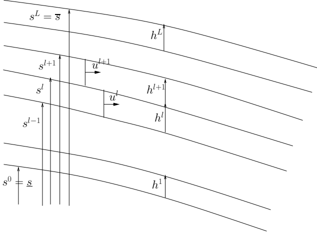
Figure 3: Multilayer splitting of the ice thickness.
