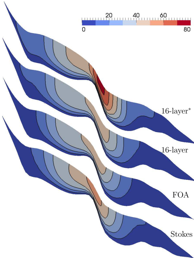
Figure 6: The horizontal velocity field across a section of Gries glacier in 1961 obtained with the 16-layer*, the 16-layer, the FOA, and the Stokes model, respectively. The unit is meters per years and the continuous lines correspond to level lines every 10 meters per year. For convenience, the horizontal domain is stretched by a factor 5.
