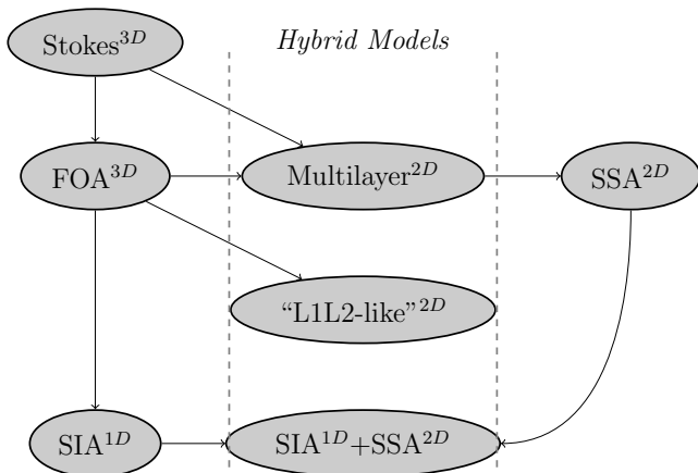
Figure 1: Overview of the hierarchy of ice flows models: Stokes, First Order Approximation (FOA), Shallow Ice Approximation (SIA), Multilayer model, “L1L2-like” and Shallow Shelf Approximation (SSA). The dimension of the mathematical model is indicated in exponent.
