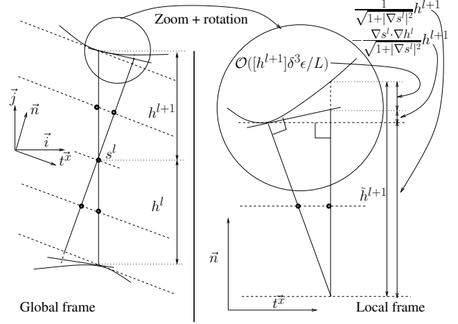
Figure 4: Representation of the global frame (left) and the local frame (right).
