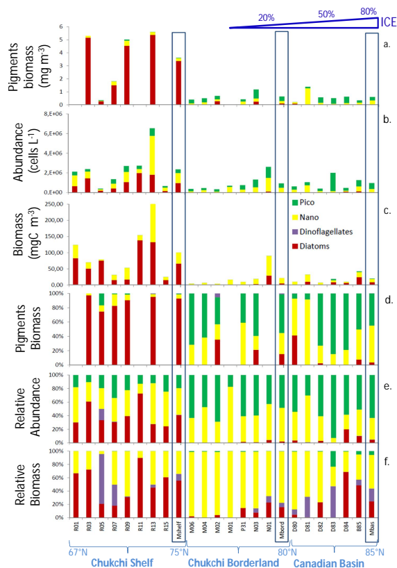
Fig. 10. Contribution of 4 major phytoplankton classes (Picoplankton, Nanoplankton, Dinoflagellates, Diatoms) in terms of (a) biomass of specific pigments allocated to each group by CHEMTAX ( \text{mg m}^{-3} ) (b) cell abundance ( \text{cells l}^{-1} ) (c) carbon biomass ( \text{mg C m}^{-3} ) and relative contribution of the 4 groups to (d) total accessory pigments biomass (%) (e) total cell abundance (%) (f) and total phytoplankton carbon biomass (%).
