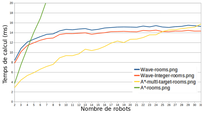
Fig. 2: A* vs wavefront for a increasing number of robots
