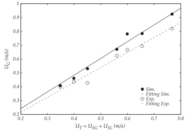
Fig. 16. Bubble velocity as a function of the mixture superficial velocity. Symbols: experimental and numerical data. Lines: linear fittings of experimental and numerical data.
