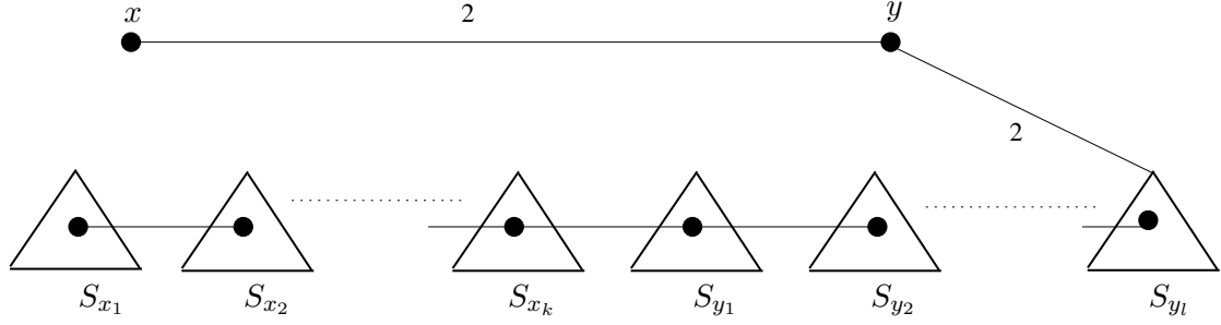
Figure 3: A Steiner tree S'' of total weight at most equal to the cost of S' .
