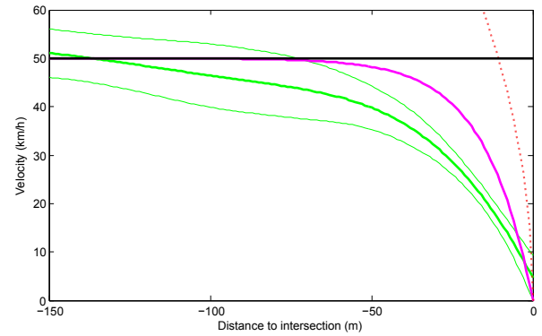
Fig. 8. Comparison of the use of a relaxed driver profile with generic average profile (generic profile in magenta, GP profile in green, the run in black and the 9\text{m/s}^2 threshold in red dots).
