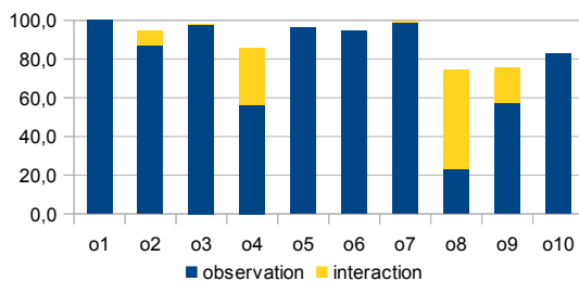
Fig. 9. Object recognition rate (with initial robot's hands appearances): the results after objects observation are shown by the blue color, and the improvement after manipulation is shown by the yellow color.
