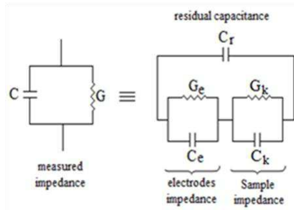
Fig. 1: Schematic representation of the equivalent circuit for measuring dielectric properties.
