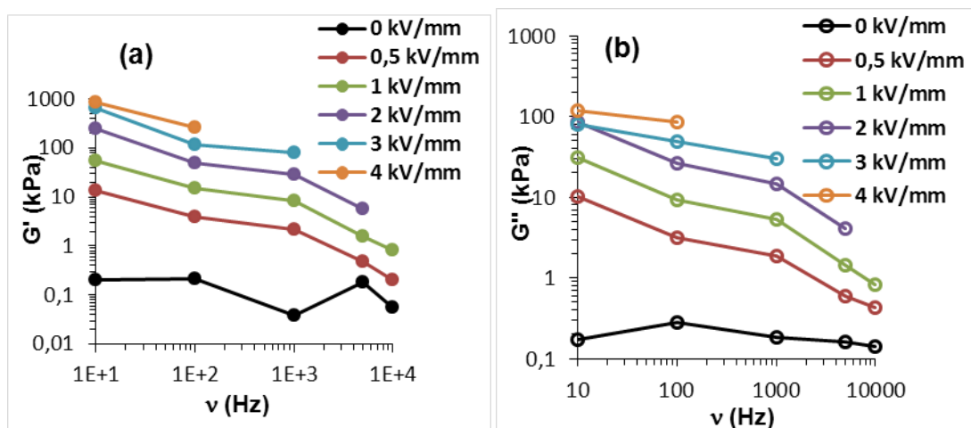
Fig. 5: Elastic modulus G' (a) , and loss modulus G'' (b) versus electric field frequency at various applied electric fields of \text{TiO}_2 -Acac/PDMS ER fluid.
