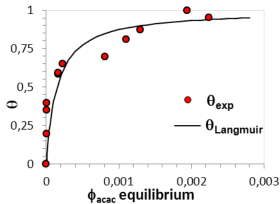
Fig. 8: Acac/TiO 2 in PDMS adsorption isotherm giving surface coverage \vartheta versus the free Acac volume fraction at equilibrium in PDMS compared to that calculated through Langmuir equation.
