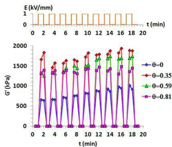
Fig. 10: Reversibility test; Elastic modulus G' versus the switching electric field between 0 and 1\text{kV/mm} ( \nu=10\text{Hz} ) successively, for different amount of Acac adsorbed on \text{TiO}_2 surface.
