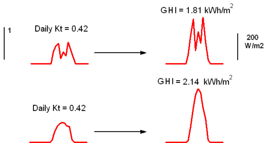
Fig. 2. Two hourly K_t series, having identically daily K_t value, provides different GHI daily values
