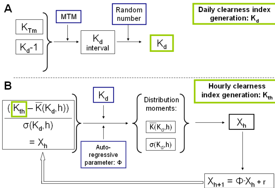
Fig. 1. Generation of synthetic daily sequences of hourly radiation values requiring as input only monthly clearness index.
