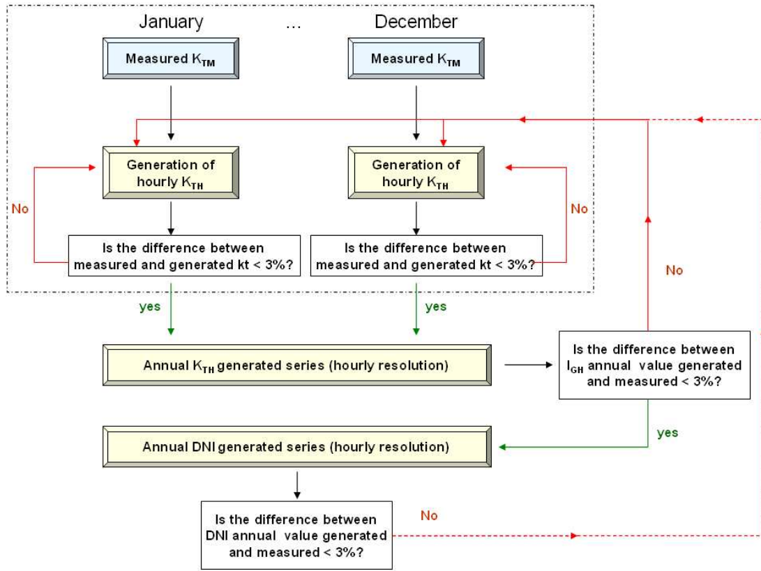
Fig. 3. GHI and DNI synthetic generation procedure.
