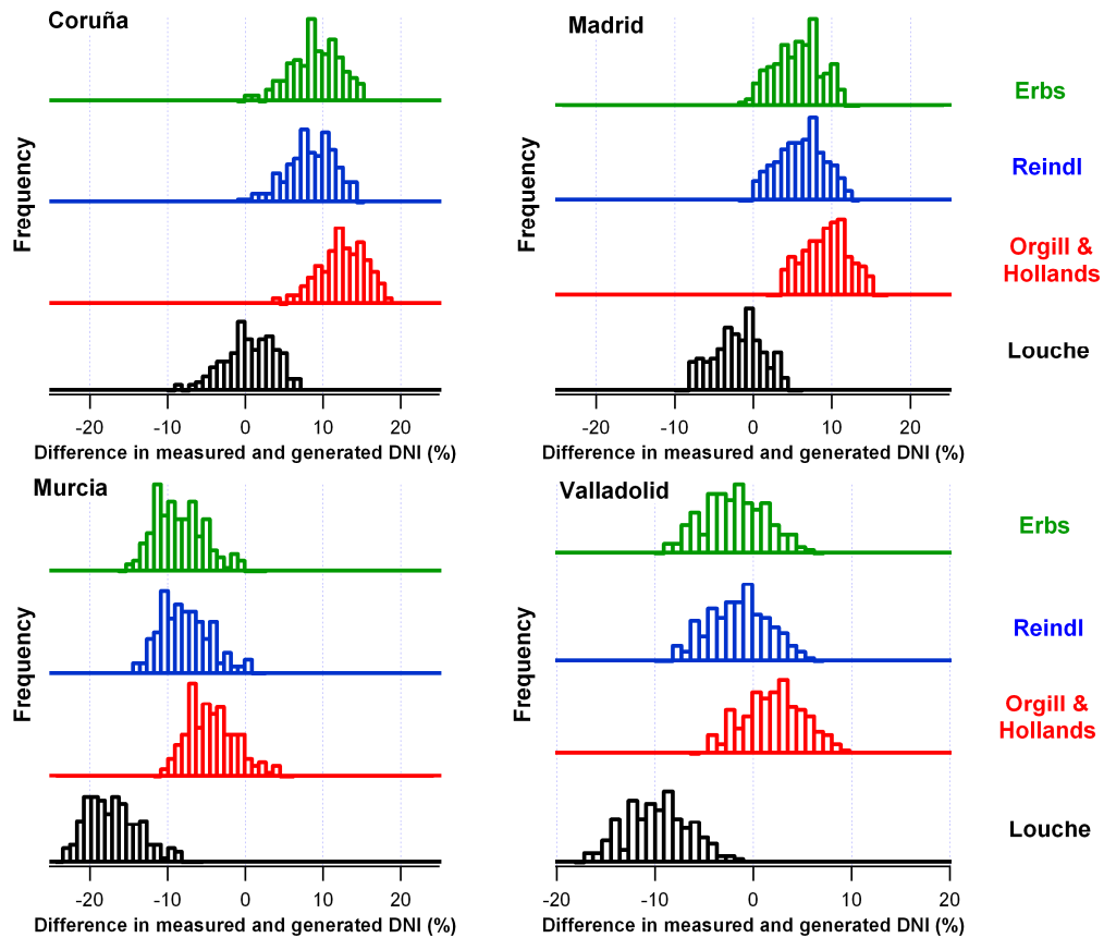
Fig. 5. Difference between measured and generated annual DNI values for each location investigated.
