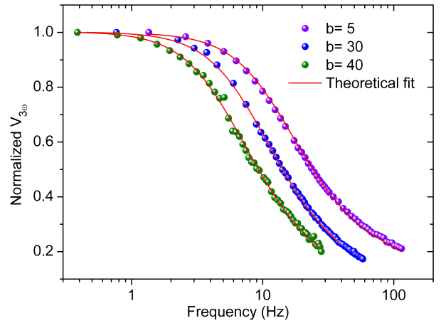
FIG. 4. V_{3\omega} voltage measurements versus frequency at 250 K using different thermometer width for a 100 nm thick membrane.
