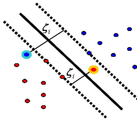
Fig. 5. Soft margin. Slaks variables.
