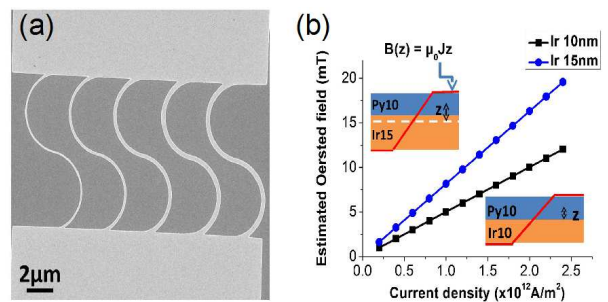
FIG. 1. (a) SEM image (Topography) of 20 \mu\text{m} long, 100 to 400 nm wide S-shaped nanostraps together with the injection pads (b) In-plane Oersted field ( B ) as a function of current density for 10 nm of Py and Ir thicknesses of 10 and 15 nm. The field value corresponds to the average field acting on the Py layer, i.e. the field in the center of the Py layer. The red lines in the insets show the Oersted field profile across the Py thickness and the dotted white line indicates the center of the Py(10nm)/Ir(15m) structure.
