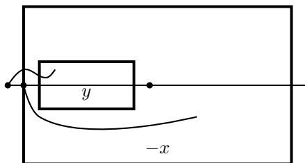
Figure B.12: The construction of \Psi(x, y) .
