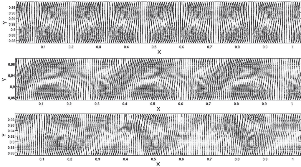
Fig. 11 – Instantaneous velocity fields on a meridional plane ( xy ) at Reynolds numbers (from top to bottom) Re = 140, 200 and 800 ( \eta = 0.85 ).
