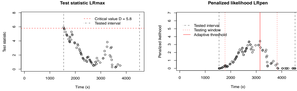
Figure 7. For the placebo group of PBC data we display the test statistics LR_{\max}(T_k|z) as function of T_k (left) and LR_{\text{pen}}(T_{\widehat{k}}, T_l|z) as function of T_l (right). The tested interval and the testing window are given by [T_{\widehat{k}}, T_{k_0}] and [T_{(1-\delta'')\widehat{k}}, T_{\delta'\widehat{k}}] respectively. The critical value D is fixed to 5.8.
