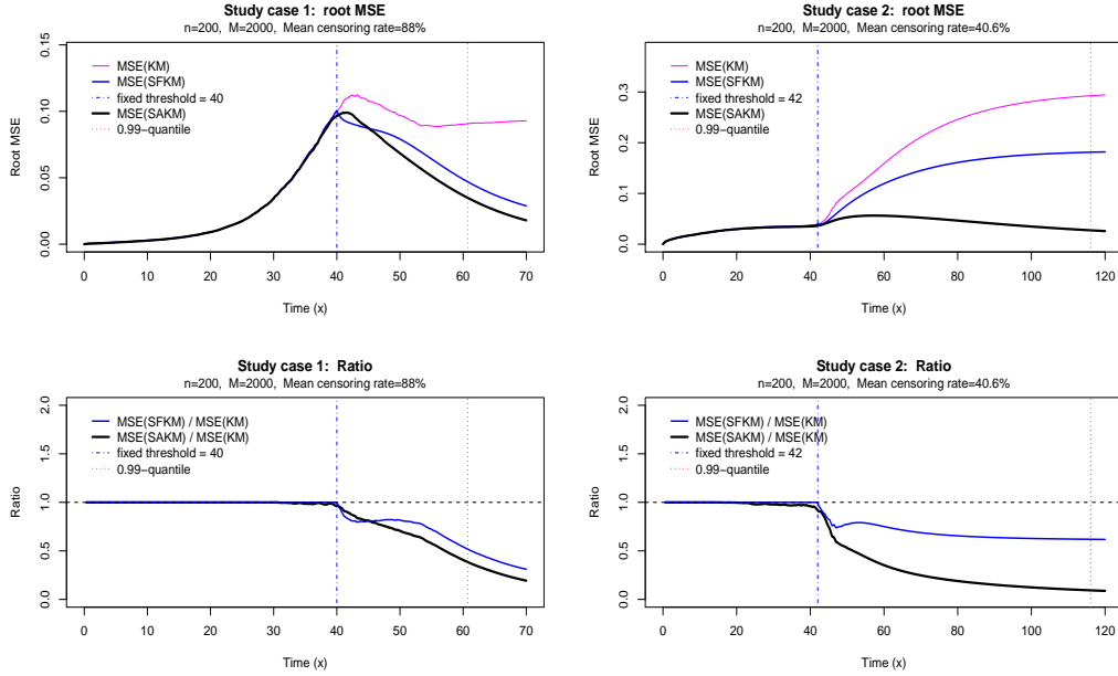
Figure 5. The top line displays the root (of type II) MSE's of three estimators: \hat{S}_{KM} (KM), \hat{S}_t (SFKM) and \hat{S}_{\hat{t}_z} (SAKM). The bottom line displays the corresponding ratios of the root MSE's on the top line. The critical value D in the SAKM is set to 6.
