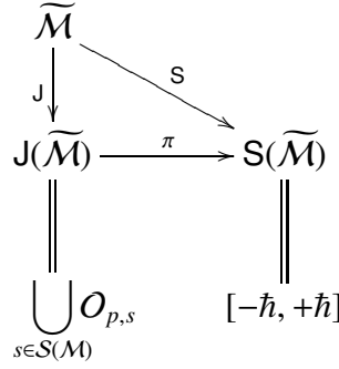
Figure 3: Double fibration of space \widetilde{\mathcal{M}} of polarized light rays
