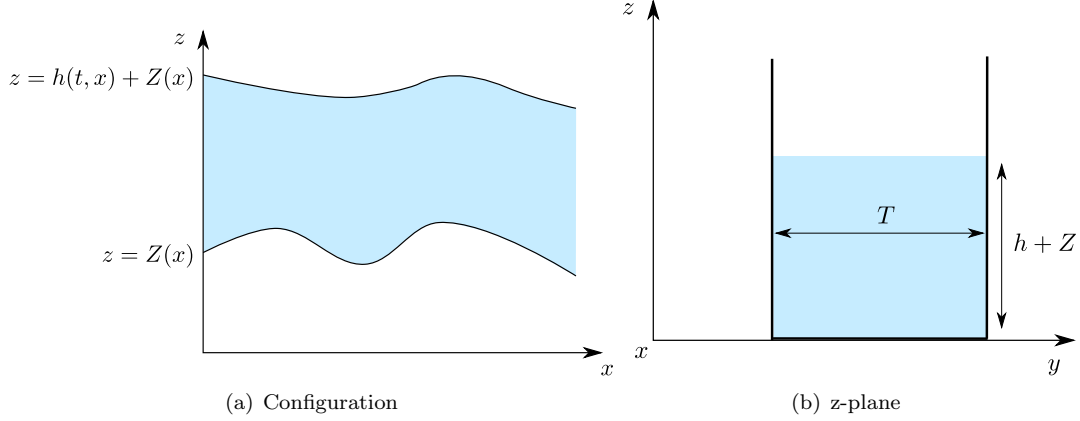
Figure 1: Geometric characteristics
