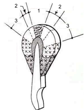
(c) Hammer head needling zones. Zone 1 : weak - light needling for piano dynamics. Zone 2 : medium - deep needling for mezzo-forte dynamics. Zone 3 : heavy - deep needling for forte dynamics. From [19].
