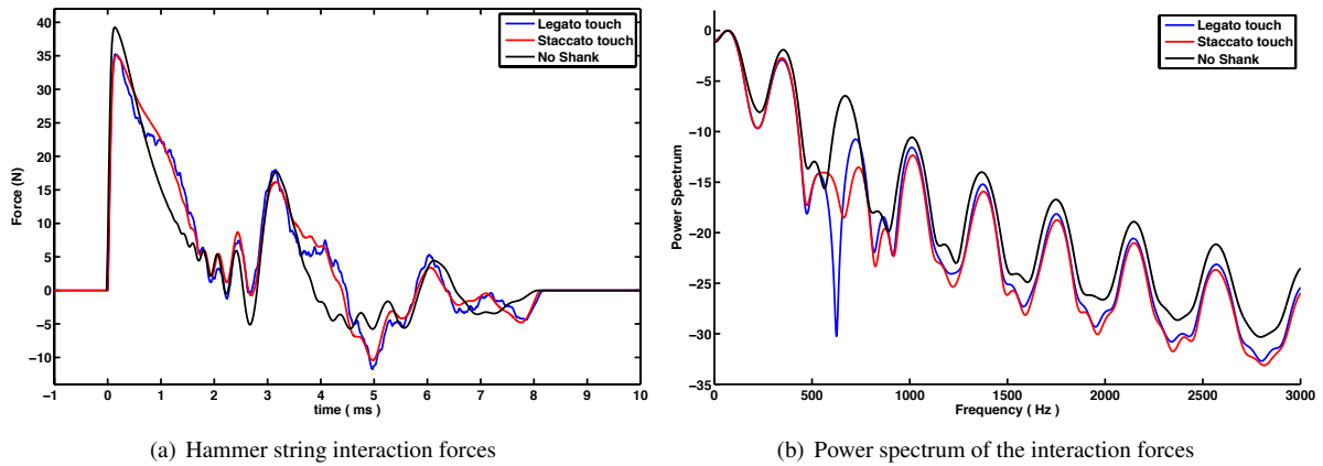
Figure 7: Temporal and spectral profiles of hammer head - string interaction forces obtained with different pianistic touches. The time scale has been shifted so that time 0 corresponds to the contact instant between the hammer head and the string.
