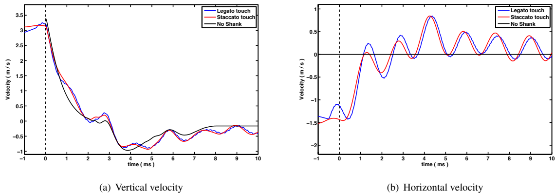
Figure 10: Velocity of the hammer head for Legato and Staccato touches. The time scale has been shifted so that time 0 corresponds to the contact instant between the hammer head and the string.
