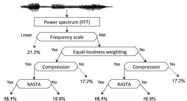
Figure 1: First stages in processing pipelines for the computation of standard MFC and PLP coefficients. The MP-ABX error rate for the PaT minimal pair discrimination task is in italics . The best pipelines are shown with plain arrows, and the best scores are underlined. Parts of the pipeline not shown are indicated by dashed arrows and the best error rate achieved in each hidden part is indicated next to the arrow.
