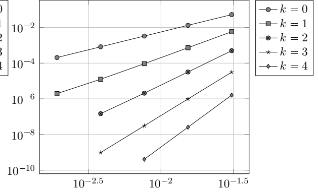
(b) \|\hat{u}_h - u_h\| vs. h , triangular mesh family
