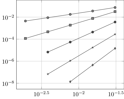
(a) \|\hat{\sigma}_h - \sigma_h\|_H vs. h , triangular mesh family
