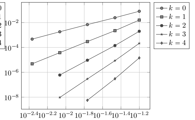
(f) \|\hat{u}_h - u_h\| vs. h , hexagonal mesh family
