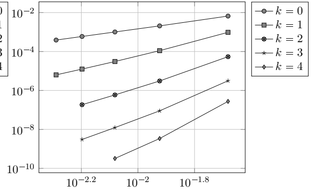
(d) \|\hat{u}_h - u_h\| vs. h , skewed quadrangular mesh family
