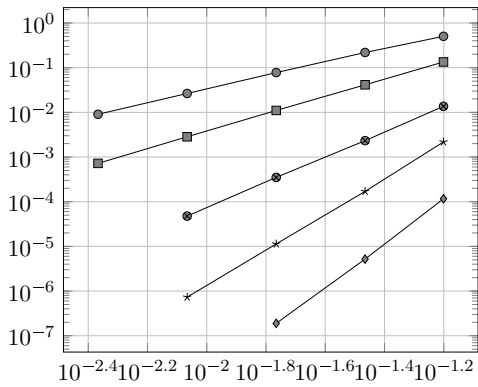
(e) \|\hat{\sigma}_h - \sigma_h\|_H vs. h , hexagonal mesh family
