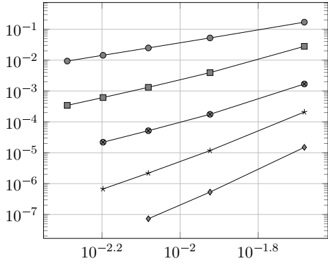
(c) \|\hat{\sigma}_h - \sigma_h\|_H vs. h , skewed quadrangular mesh family
