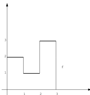
FIGURE 4. Function f
