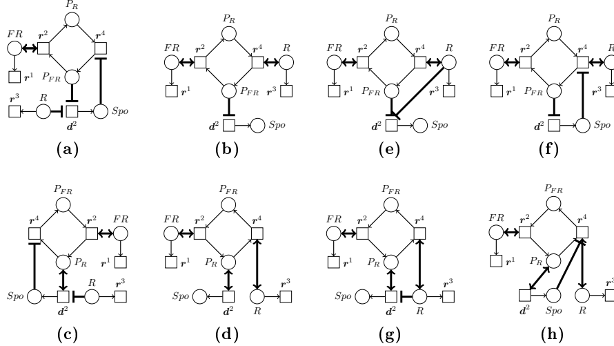
Fig. 3. The eight \mathcal{X}' -deterministic extended Petri nets resulting from \mathcal{P}_{S_4} .
