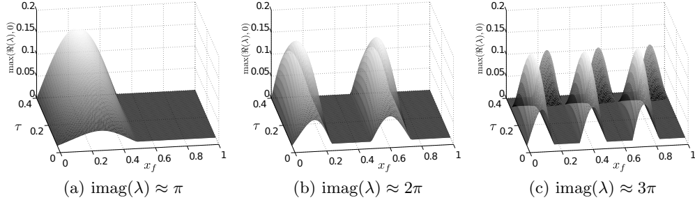
Figure 5: The region of instability for the first three frequency modes ( K = 0.8 ) for the analytical solution.
