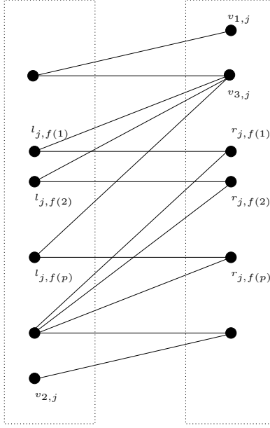
Figure 3: The gadget H(x_j) .
