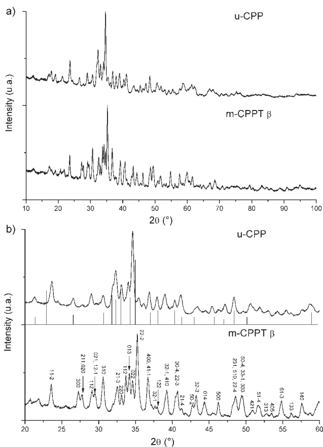
Fig. 2 XRD patterns of the two hydrated calcium pyrophosphate phases synthesised using two different setups: a) in the 2\theta = 10\text{--}100^\circ domain; b) in the 2\theta = 20\text{--}60^\circ domain (bars under u-CPP diagram correspond to the diagram of h-CPPD phase reported by Mandel 2 ).
