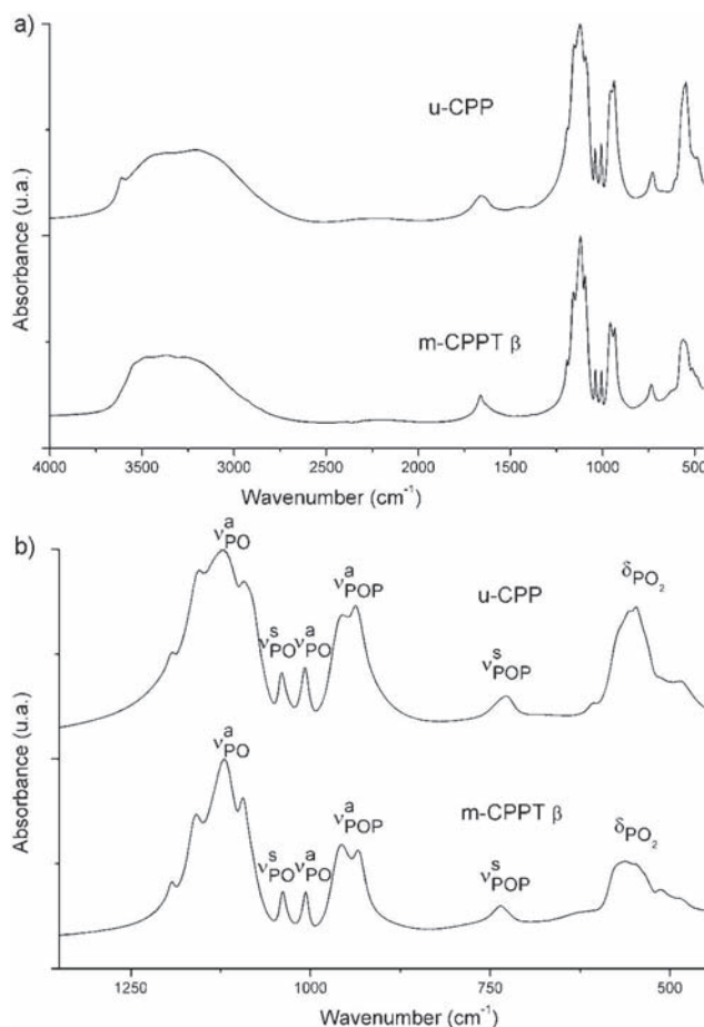
Fig. 4 FTIR spectra of the two hydrated calcium pyrophosphate phases synthesised in the same conditions but using two different setups: m-CPPT \beta and u-CPP: a) 4000 – 400\text{ cm}^{-1} domain; b) 1300 – 500\text{ cm}^{-1} domain.
