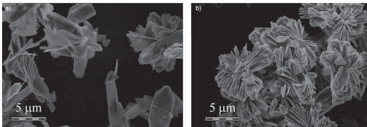
Fig. 3 SEM micrographs of the two hydrated calcium pyrophosphate phases synthesised under the same conditions but using two different setups: a) m-CPPT \beta ; b) u-CPP.
