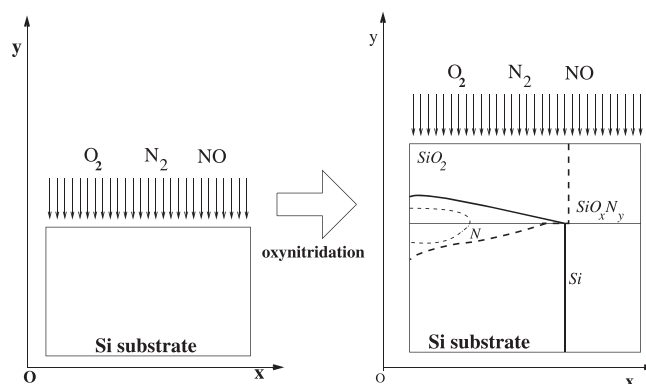
FIG. 6. Schematic view of the system model. The profile of Si, SiO_2 , and nitrogen concentration are presented and lead to the definition of two different layers: the oxynitride SiO_xN_y and the Si part.
