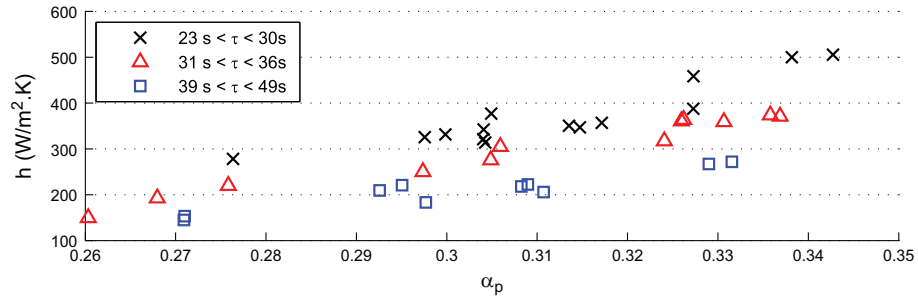
Fig. 12. Average heat transfer coefficient as a function of the average particle volume fraction.
