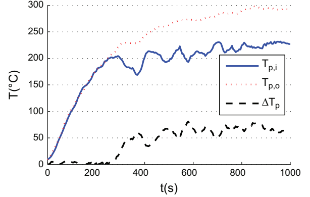
Fig. 6. Solid temperature as a function of time in the irradiated cavity (operating conditions: average solid superficial mass-flow rate = 12.28 \text{ kg/m}^2 \text{ s} ; aeration = 0.109 \text{ sm}^3/\text{m}^2 \text{ s} ; solar flux density = 223 \text{ kW/m}^2 ).
