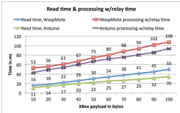
Fig. 7. Measured time to read data
