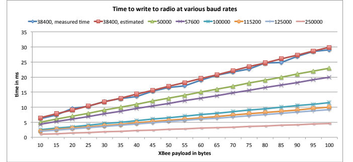
Fig. 3. Time to write to radio at various baud rates
