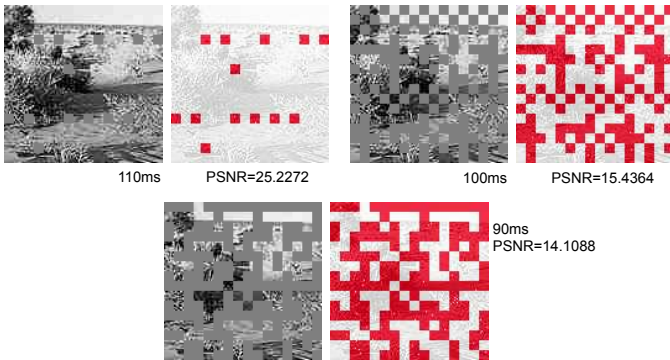
Fig. 11. 128x128 image received, Libelium WaspMote relay
