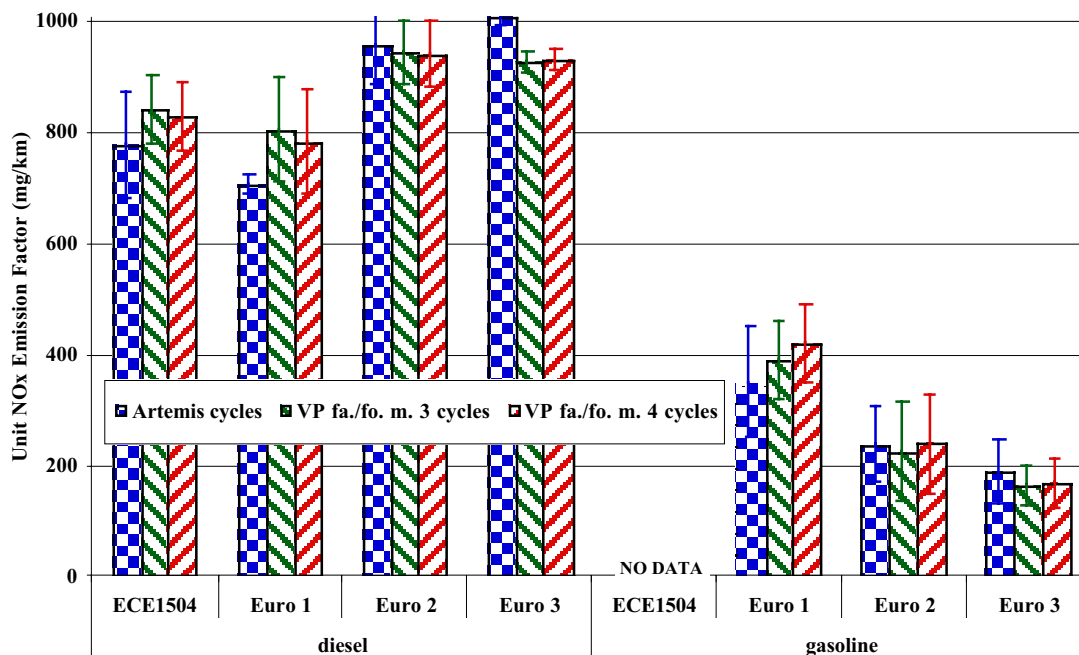
Figure 3: Progression of NOx emission factor with regulation.
