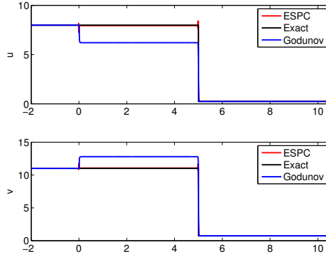
Figure 4.15. Comparison of the ESPC and Godunov schemes for the coupled Burgers system (4.1) with the exact solution.
