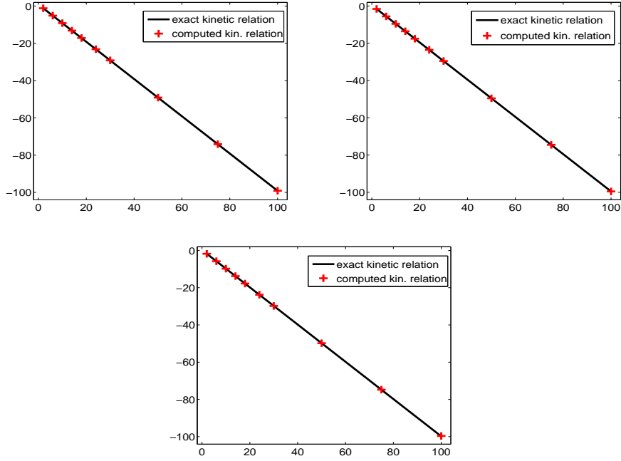
Figure 3.7. Intermediate state (kinetic function) (Y-axis) for the cubic conservation law for varying left-hand state u - L (X-axis), computed using an eighth-order WCD scheme with \tau = 0.1 . Left: Kinetic function for \delta = 0.3 . Middle: Kinetic function for \delta = 1 . Right: Kinetic function for \delta = 5 .
