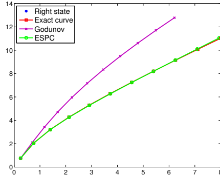
Figure 4.16. Numerical Hugoniot locus for the coupled Burgers equation (4.1) generated by the ESPC and Godunov schemes, compared with the exact Hugoniot locus.
