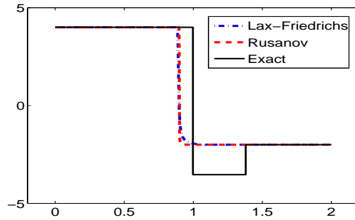
Figure 3.1. Approximation of small-scale dependent shock waves for the cubic conservation law with vanishing diffusion and capillarity (2.5) using the standard Lax-Friedrichs and Rusanov schemes
