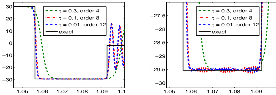
Figure 3.5. Convergence p \rightarrow +\infty (increasing order of the scheme) for the WCD scheme for a moderate shock. Left: Solution of the Riemann problem for u_L = 30 . Right: Closer view of the middle state u_M .
