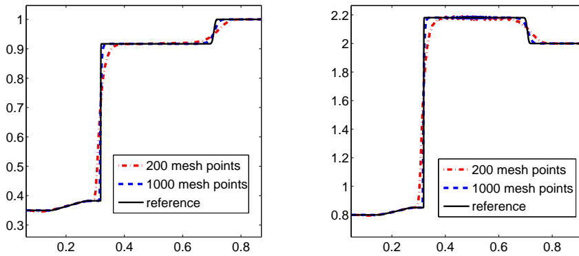
Figure 3.8. Mesh-convergence for the WCD scheme for the dispersive limit of van der Waals fluid with initial data (3.22) with a eighth-order WCD scheme.
