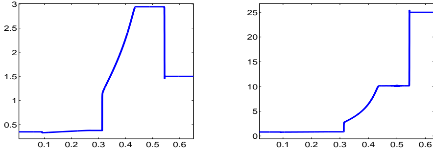
Figure 3.10. Approximation of the Riemann solution with initial data (3.23) resulting in a large jump in volume \tau .
