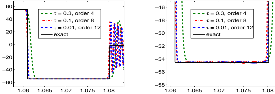
Figure 3.6. Convergence p \rightarrow +\infty for a large nonclassical shock for the cubic conservation law. Left: Solution of the Riemann problem for u_L = 55 . Right: Closer view of the middle state u_M .
