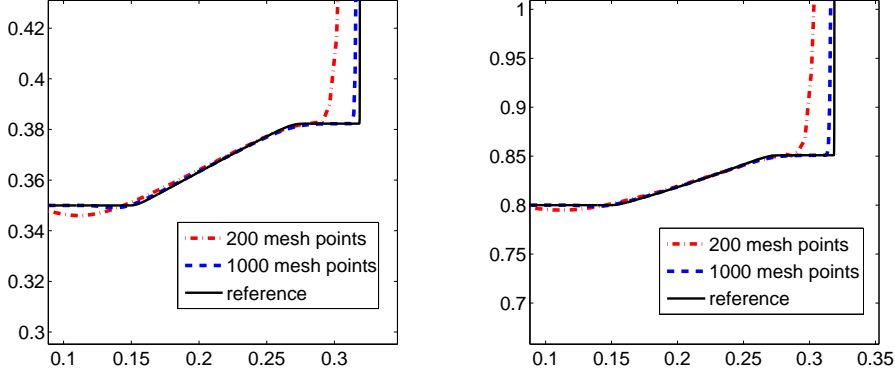
Figure 3.9. Zoom near nonclassical states for the dispersive limit of van der Waals fluid with initial data (3.22) and a eighth-order WCD scheme.
