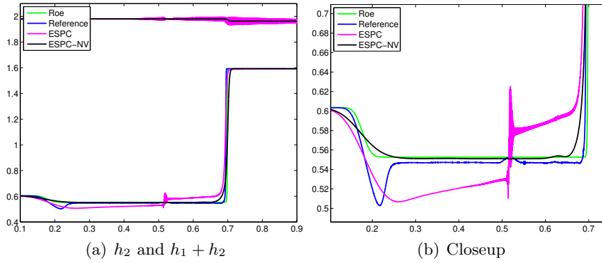
Figure 4.17. Approximate solutions for height of bottom layer ( h_2 ) and total height ( h_1 = h_2 ) for the two-layer shallow water system (4.2) with the ESPC, ESPC-NV and path-consistent Roe schemes. A reference solution, computed from the viscous shallow water system (4.21) is also displayed.
