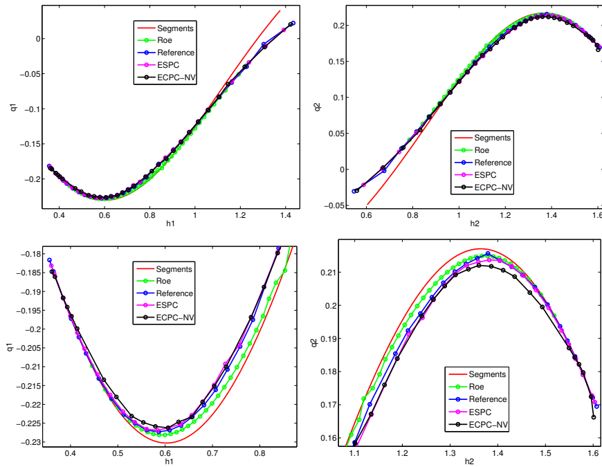
Figure 4.18. Hugoniot loci in the h_1 - (h_1u_1) and h_2 - (h_2u_2) planes for the two-layer shallow water equations (4.2), computed with the ESPC, ESPC-NV and Roe schemes. A reference Hugoniot locus computed from the viscous shallow water system (4.21) and a Hugoniot locus computed using straight line paths are also shown.
