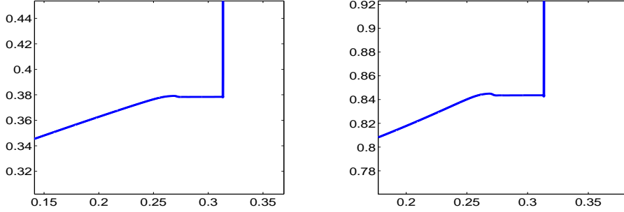
Figure 3.11. Zoom at nonclassical states in the approximation of the Riemann problem with initial data (3.23) resulting in a large jump in volume \tau .
