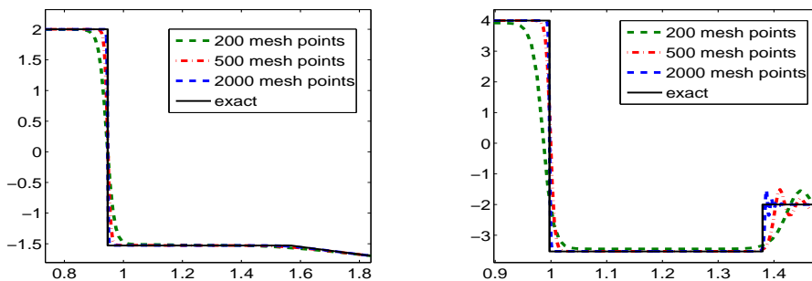
Figure 3.4. Convergence (mesh refinement) for the WCD schemes and small shocks. All approximations are based on an order 8 scheme and \tau = 0.01 . Left: Riemann solution for u_L = 2 . Right: Riemann solution for u_L = 4 .
