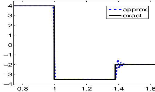
Figure 3.2. Approximation of nonclassical shocks to the cubic conservation law (with vanishing diffusion and capillarity) (2.5) using LeFloch-Mohamadian's sixth-order scheme with controlled dissipation (3.4) with c = 5
