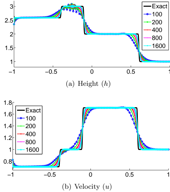
Figure 5.21. Solutions of the linearized shallow water equations (5.8) at time t = 0.25 with initial data (5.12) and boundary data (5.13) computed with the CND scheme at different mesh resolutions. The exact solution is provided for comparison.
