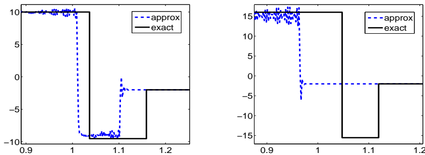
Figure 3.3. Approximation of strong nonclassical shocks for the cubic conservation law (2.5) using LeFloch-Mohamadian's sixth-order scheme with controlled dissipation (3.4) with c = 5 . Left: Initial jump = 10. Right: Initial jump = 16.
