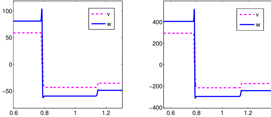
Figure 3.12. Large shocks in v and w -variable for the Hall MHD system using a fourth order WCD scheme with 4000 mesh points.
