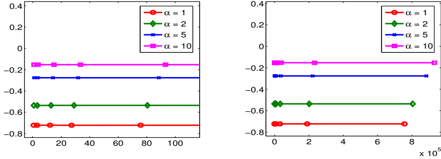
Figure 3.13. Scaled entropy dissipation \frac{\phi(s)}{s^2} vs. shock speed s for the Hall MHD model (3.24) with a fourth-order WCD scheme.
