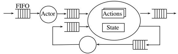
Fig. 1: A CAL network.
