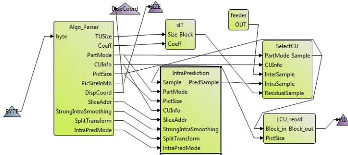
Fig. 8: HEVC intra-decoder architecture.
