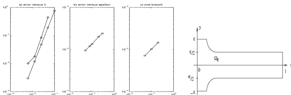
FIG. 7.2. Error between the 1D-2D approximate solution and the exact solution a) as a function of h b) as a function of \epsilon c) and d) special case one branch
