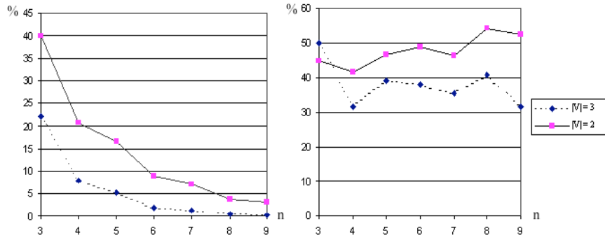
Figure 5: Ratio of Decision and Strong Convergence Vectors Against the Number of Processes
