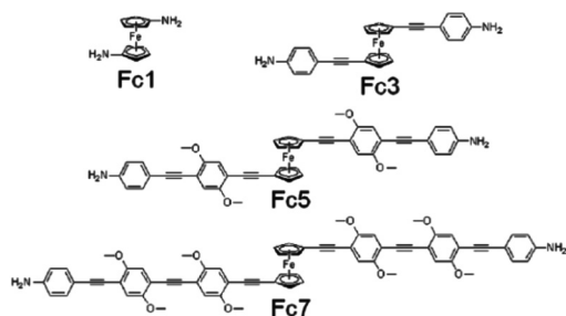
Scheme 3 Ferrocene in OPEs. Reprinted with permission from ref. 15. Copyright 2013 ACS.
