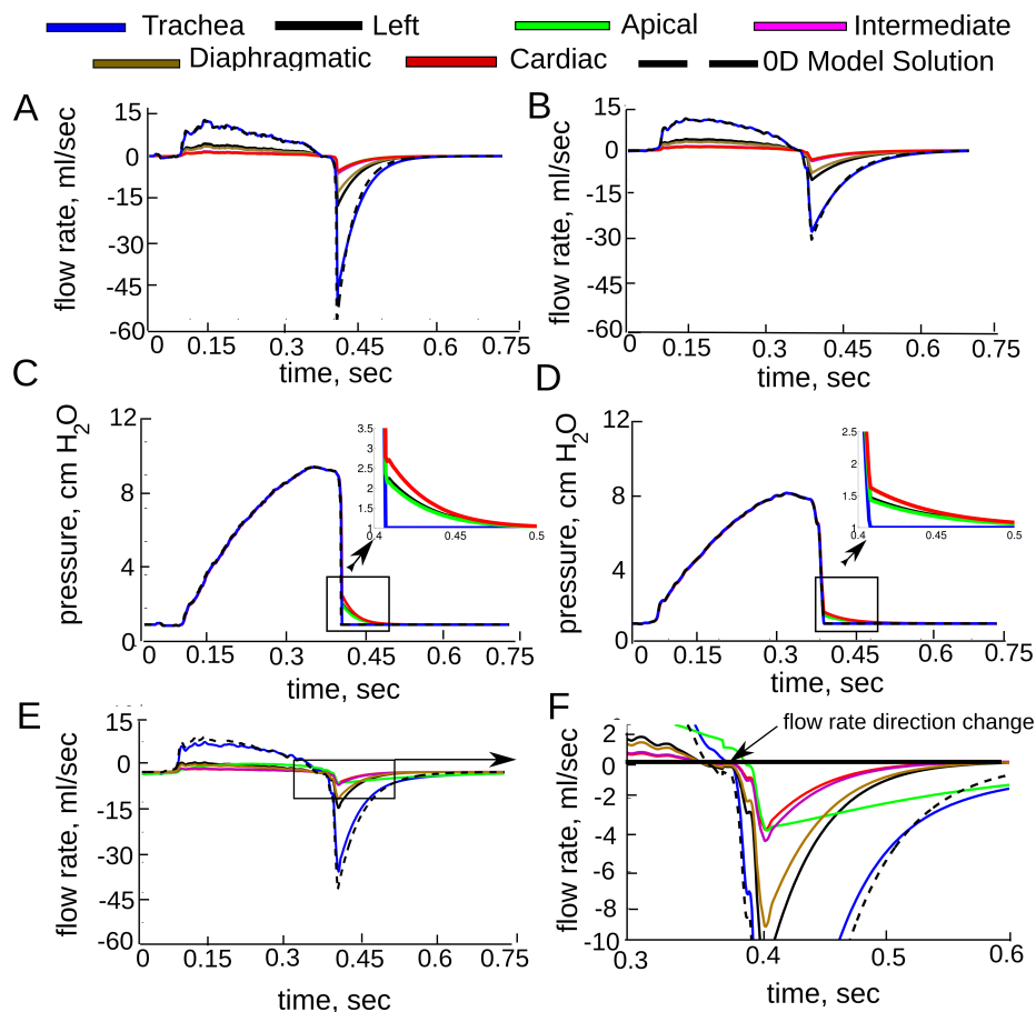
Figure 3: Computed flow rate and average pressure at each face for healthy (panels A and C), homogeneous emphysema (panels B and D) and heterogeneous emphysema (apical lobe) (panels E and F). The simulated flow rate at the trachea was similar to the 0D model solution, except during maximum exhalation where the 3D pressure drop was the greatest (shown in panels C and D). Panel F shows the delay in the flow direction change and slower emptying in the diseased lobe.
